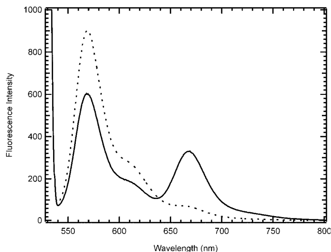
FIGURE 2 (Dotted line) Fluorescence emission spectrum of a solution containing 0.5 \mu\text{M} gA-Cy3 donor and 0.5 \mu\text{M} pF-Phe-gA-Cy5 acceptor peptides incorporated individually into separate unilamellar lipid vesicles. (Solid line) Fluorescence emission spectrum of 0.5 \mu\text{M} gA-Cy3 donor and 0.5 \mu\text{M} pF-Phe-gA-Cy5 acceptor peptides coinorporated into a single population of unilamellar lipid vesicles. Sensitized emission is evident. (Excitation at 520 nm, 10-nm excitation and emission slit widths, lipid concentration: 6.4 mM dioleoyl-phosphatidylcholine).
